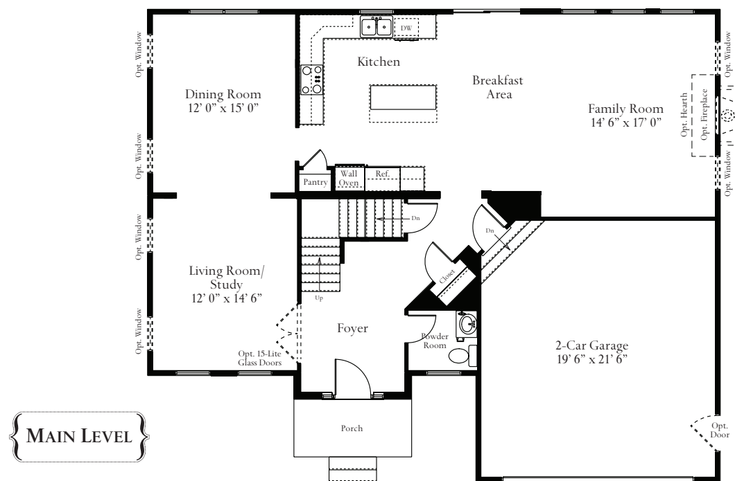
First Floor Plan with Opt. 4' Family Room Extension
